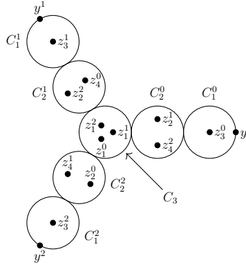
FIGURE 8. An element of \overline{\mathcal{L}}_3^4 with components labeled via Notation 5.1.
