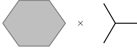
FIGURE 11. The \Delta -face F_{\mathbf{I}} \subseteq \Delta_4^3 of Example 7.8, decomposed as a product according to its (x_2, x_3, x_4) -coordinates and its x_1 -coordinate.
