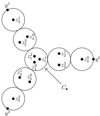
FIGURE 3. A stable length-two (4, 3) -curve, where each circle represents a \mathbb{P}^1 component and \sigma is the rotational automorphism. Not pictured are the marked points x^+ and x^- , which are the two fixed points of \sigma and must both lie on the central component C_\bullet .
