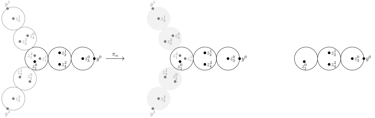
FIGURE 7. The image of the curve in Figure 3 under \pi_\alpha , where \alpha(0) = 0 , \alpha(1) \in \mathbb{Z}_3 , \alpha(2) = 1 , \alpha(3) = 0 and \alpha(4) = 2 .
