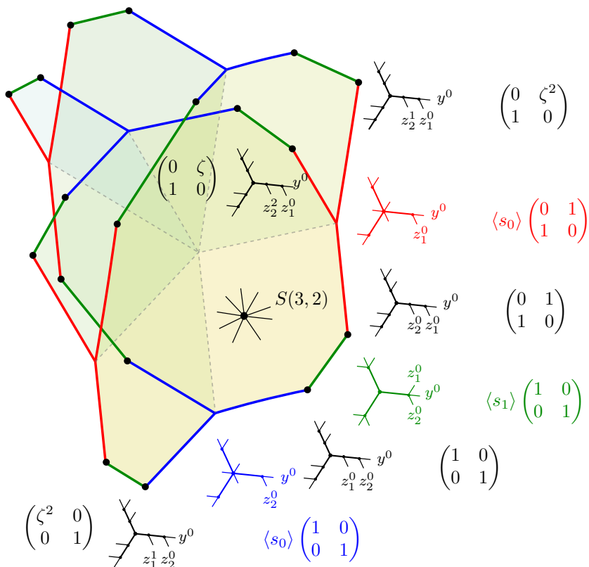
FIGURE 2. A projection of the polytope \Delta_2^3 , with some \Delta -faces labeled by both the boundary strata in \overline{\mathcal{L}}_2^3 and by the corresponding \mathcal{T} -cosets in S(3, 2) .
