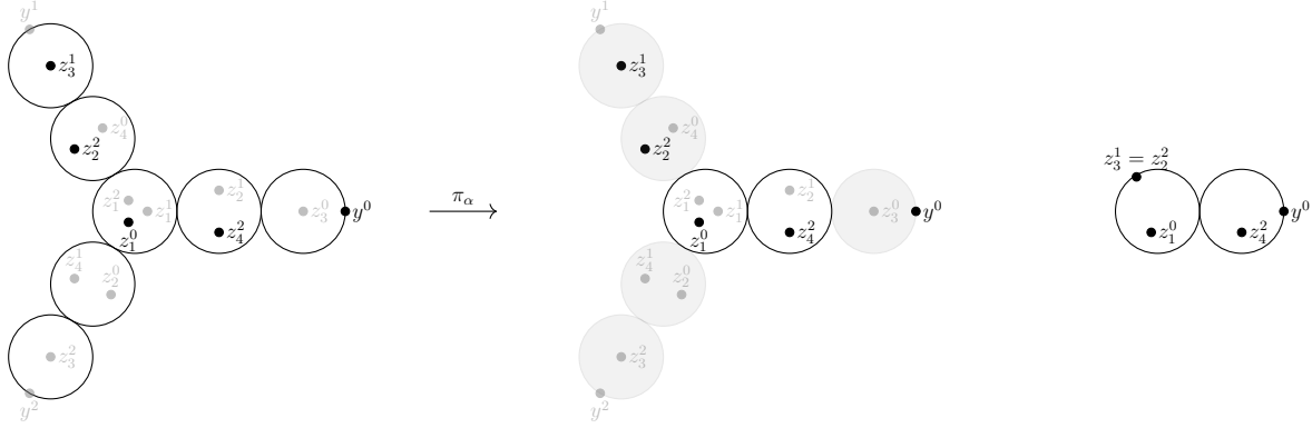
FIGURE 6. A visualization of the map \pi_\alpha in the case where \alpha(0) = 0 , \alpha(1) = 0 , \alpha(2) = 2 , \alpha(3) = 1 , \alpha(4) = 2 . The marked points x^\pm are on the central component and are not pictured. The faded marked points are forgotten under \pi_\alpha and the faded solid circles indicate contracted components as a result of forgetting some of the marked points.
