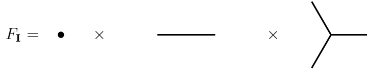
FIGURE 10. The \Delta -face F_{\mathbf{I}} \subseteq \Delta_{\mathbf{4}}^3 of Example 7.7, decomposed as a product according to its x_3 -coordinate, its (x_2, x_4) -coordinates, and its x_1 -coordinate.
