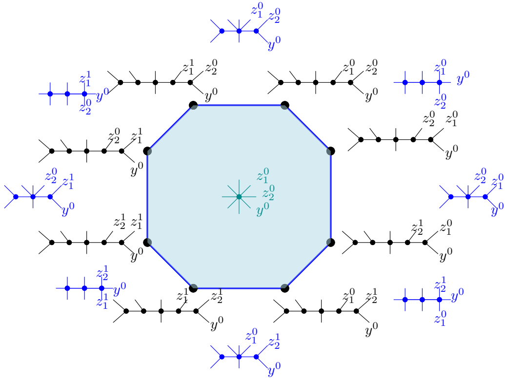
(A) The polytope \Delta_2^2 with faces labeled by boundary strata in \bar{\mathcal{L}}_2^2 . The markings on the left side of each stratum are omitted for clarity but are uniquely determined by the involution.
