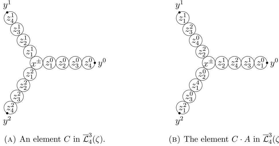
FIGURE 12. The action of A \in S(3, 4) defined by (33) on an element of \overline{\mathcal{L}}_4^3(\zeta) .
