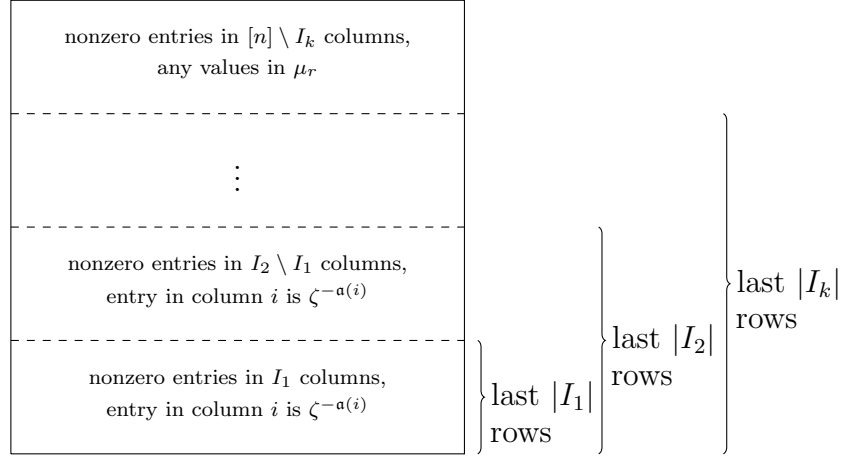
FIGURE 9. A typical element of the \mathcal{T} -coset C_{\mathbf{I}} . The action of H_{\mathbf{I}} permutes rows within each of the blocks separated by dotted lines, and multiplies elements of the top-most block by r th roots of unity.
