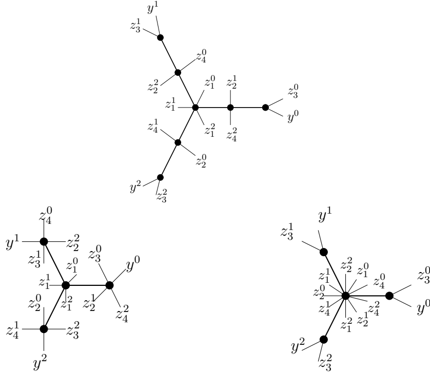
FIGURE 4. The dual graph G of the curve in Figure 3, and below it, the dual graphs of two other curves in the boundary stratum S_G , corresponding to two edge-contractions of G .
