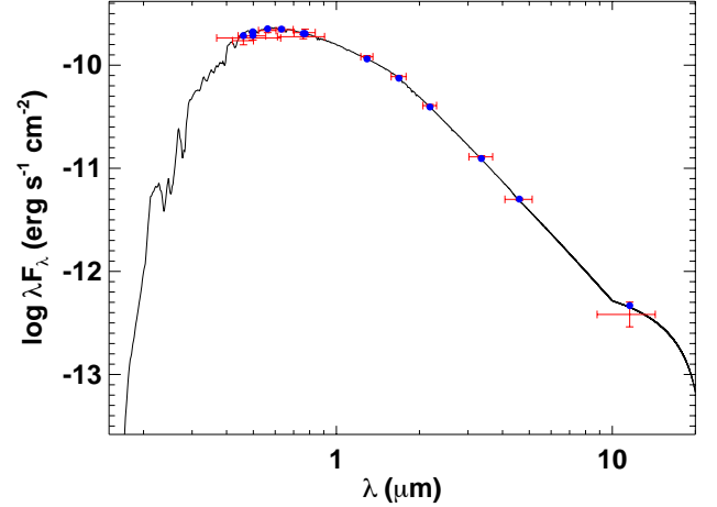
Fig. 4. Spectral energy distribution (SED) for TOI-5542. Red symbols represent the observed photometric measurements, where the horizontal bars represent the effective width of the passband. Blue symbols are the model fluxes from the best-fit Kurucz atmosphere model (black).
