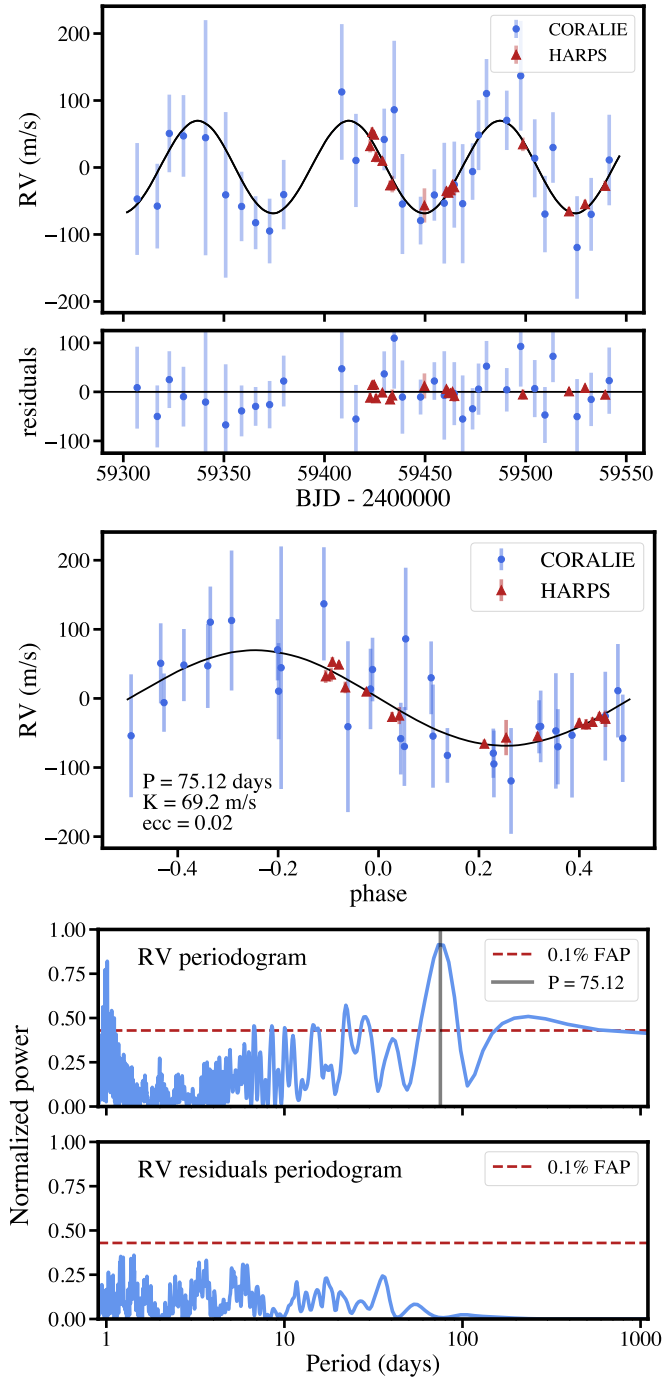
Fig. 3. CORALIE and HARPS RVs, as described in Sect. 2. Top plot shows the full time baseline of the RV observations, while the middle plot shows the RVs phased to the 75.12 day period. The black lines show the best-fit Keplerian model to the RVs from our juliet analysis, as described in Sect. 3.2. Lower plot shows the Lomb-Scargle periodogram of the original data as well as the residuals. Red dashed lines show a false alarm probability (FAP) of 0.1%.
