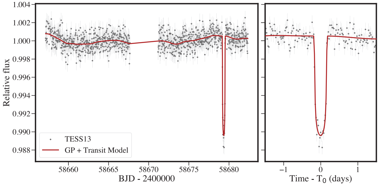
Fig. A.1. Full TESS Sector 13 data of TOI-5542 . Zoom-in on transit shown on the right. The black circles display the 30-min SPOC data used in the analysis and the red line displays the full GP and transit model.
