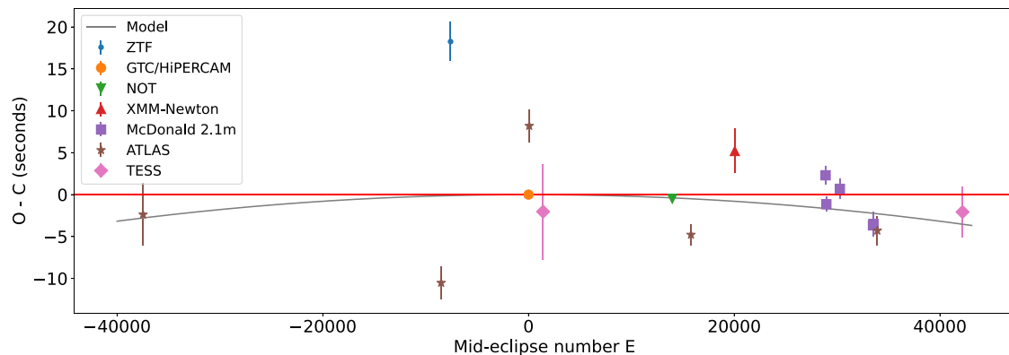
Figure 8. The theoretical O - C for ZTF J2130 obtained using \dot{P} from Kupfer et al. (2020a) (grey curve) shown along with the observed O - C values from our data.
