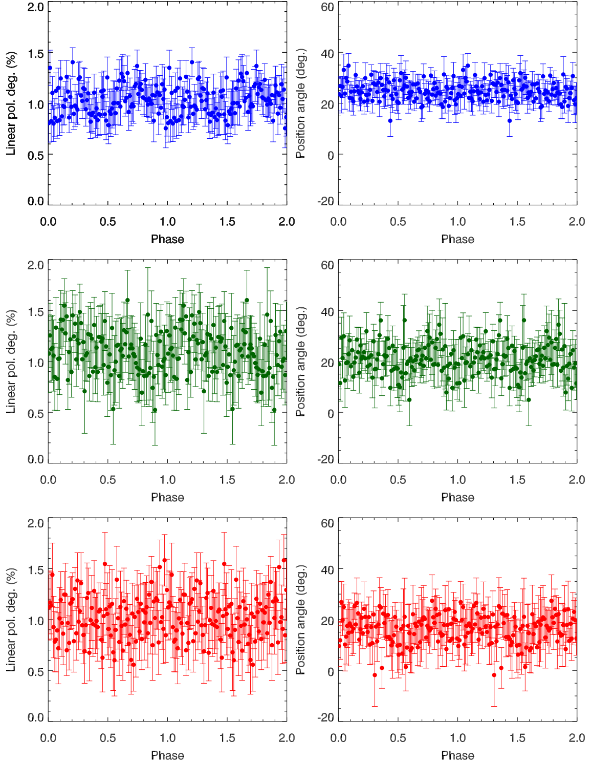
Figure 3. NOT/DiPol-UF B'V'R' polarimetry of ZTF J2130. The colours correspond to BVR bands (top to bottom). The data are shown twice for clarity.
