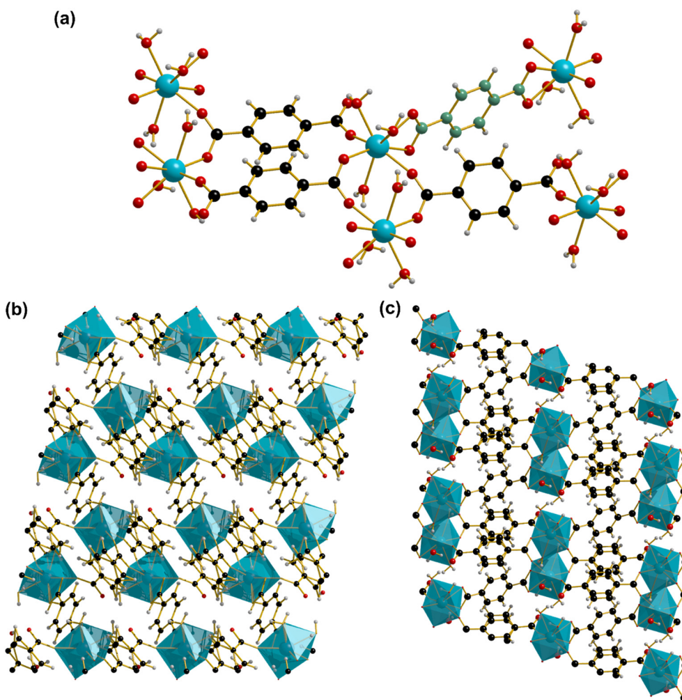
Fig. 3 The structure of UOW-3. (a): Coordination geometry around the blue \text{Yb}^{\text{III}} centre depicting the three partially uncoordinated 'type 2' BDC linkers in black, the fully coordinated \eta^2 symmetrical BDC linker in green and each of the directly connected \text{Yb}^{\text{III}} centres shown with their complete coordination spheres. (b): The overall structure of UOW-3 viewed along the [001] direction, with isolated \text{Yb}^{\text{III}} ions depicted as blue polyhedra, and narrow channels with carboxylates depicted protruding into the pores. (c): The structure of UOW-3 viewed along the [100] direction showing the pseudo, pillared layered structure.
