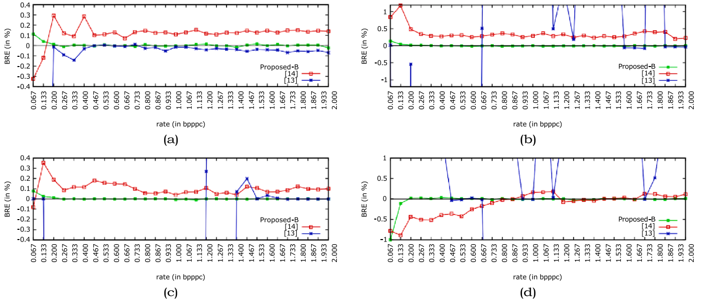
Fig. 6. Average BRE values (in %) of the evaluated approaches for 30 bitrates (bppcc). (a) SKNF6, (b) END1, (c) LNGF1, and (d) PANC5.
