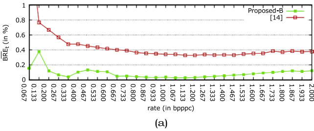
Fig. 7. \overline{BRE}_t (in %) averaged for all the images for the Proposed-B and [22].
