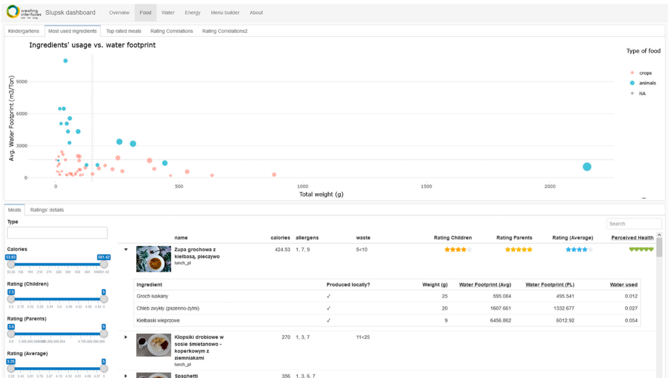
Fig. 7. Scatter plot comparing average water footprint (y-axis), usage (total weight, x-axis) and total consumption (size) by ingredient and ingredient type (colour).
