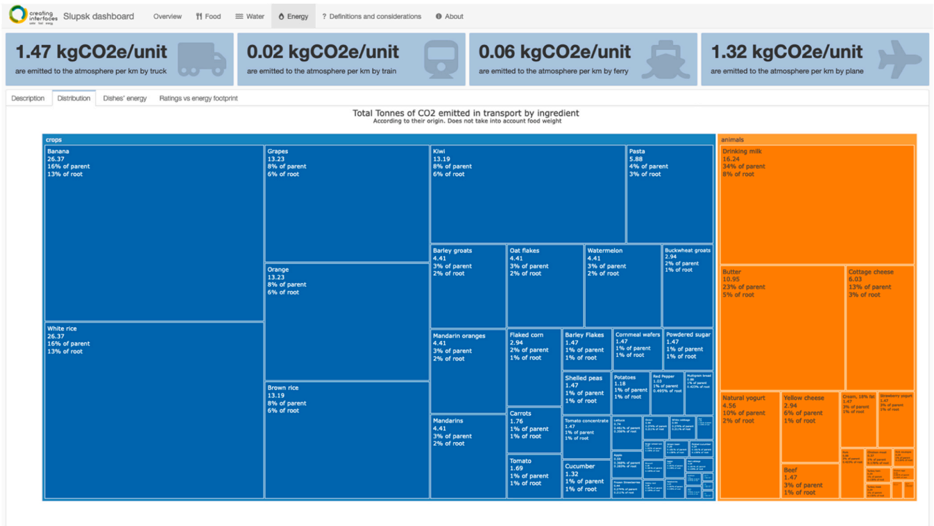
Fig. 6. Treemap displaying ingredients' energy consumption and how they compare in relation to the total. Size represents CO2 emitted in transport by ingredient, colour ingredient's origin (animal -orange- vs plant-based -blue).
