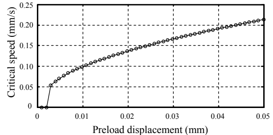
Fig.5. Effect of preload on critical scanning speed
