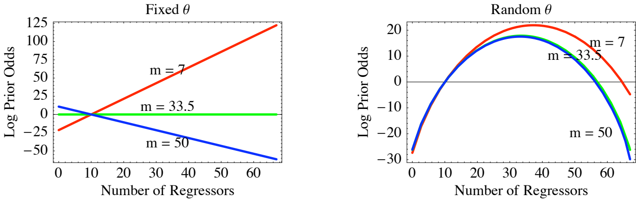
Fig. 2. Log of Prior Odds: k_i = 10 vs varying k_j . The left panel is for fixed \theta and the right panel for random \theta .
