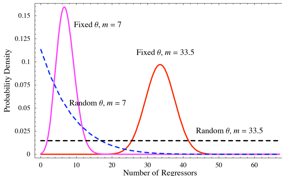
Fig. 1. Prior model size for fixed \theta (solid) and random \theta (dashed), with m = 7 and m = 33.5 .
