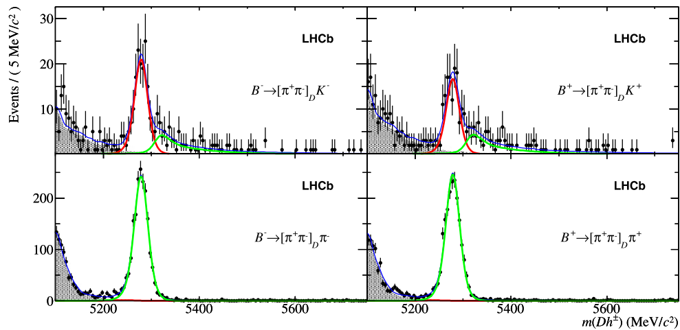
Fig. 3. Invariant mass distributions of selected B^\pm \rightarrow [\pi^+\pi^-]_D h^\pm candidates. See the caption of Fig. 1 for a full description.
