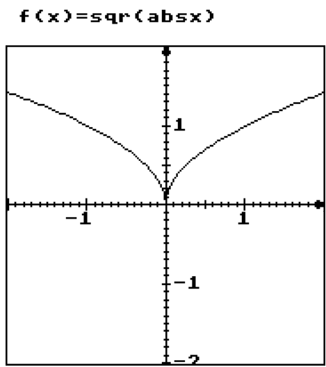
Figure 12: The graph of y=\sqrt{|x|} – does it have a tangent at the origin?
