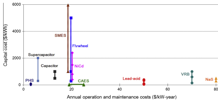
Fig. 18. Comparison of energy capital cost and annual operating &amp; maintenance cost.
