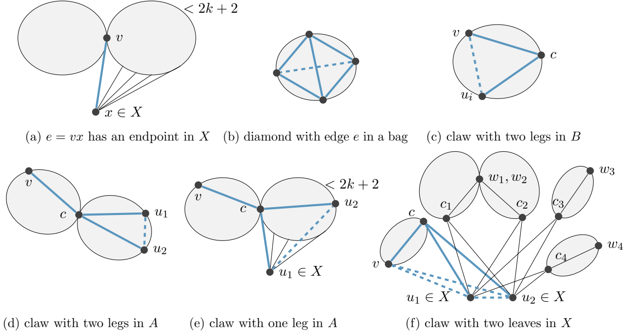
Figure 3: The different situations where a claw or diamond (thick blue edges and dashed non-edges) might appear in G - F' , each leading to a contradiction.
