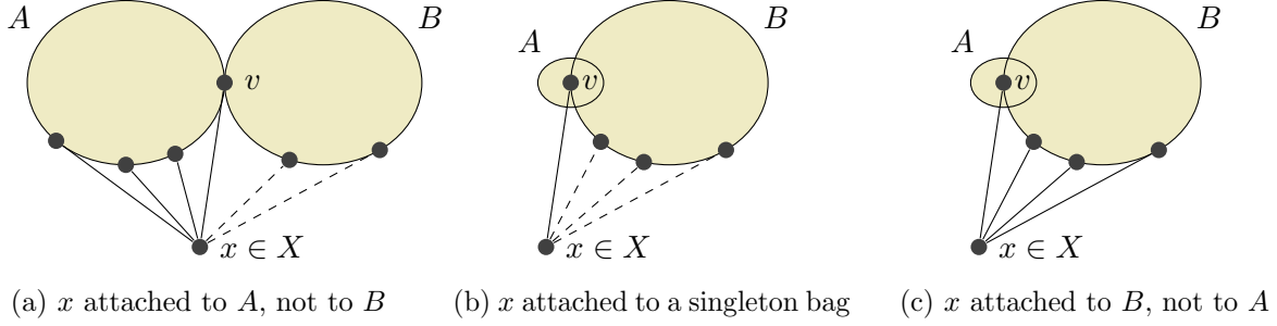
Figure 1: Possible ways in which a vertex in X can neighbor a vertex v in G - X and the two bags containing it.
