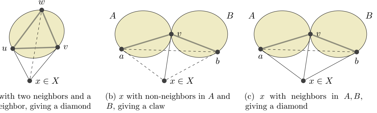
Figure 2: Adjacencies between X and G - X that lead to a contradiction.
