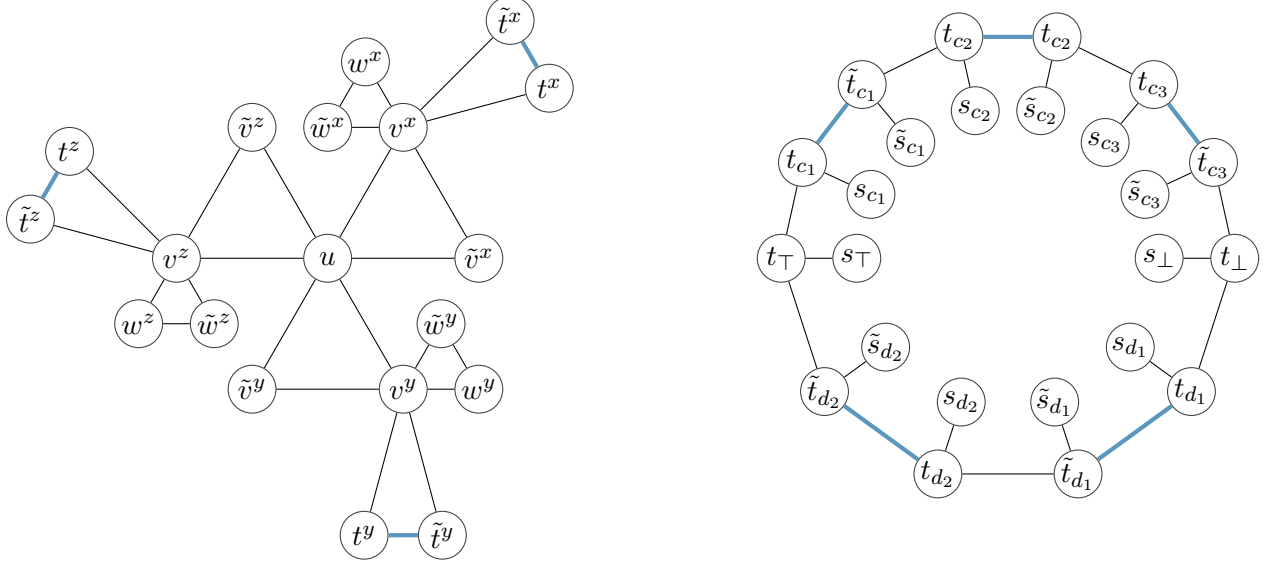
Figure 4: The clause gadget G_c (left) and variable gadget G^x (right) used in the reduction.
