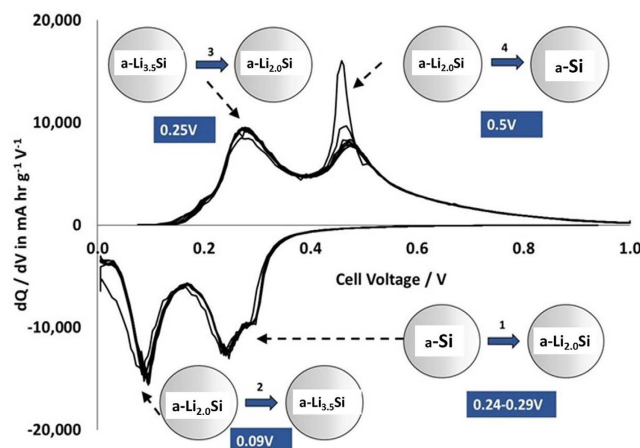
Figure 9. Differential capacity analysis ( dQ/dV ): the first derivative of the galvanostatic curve over cycles 2–10. Each peak is accompanied by diagrams explaining the structural transformations that are taking place within the anode as a function of the highlighted voltages.
