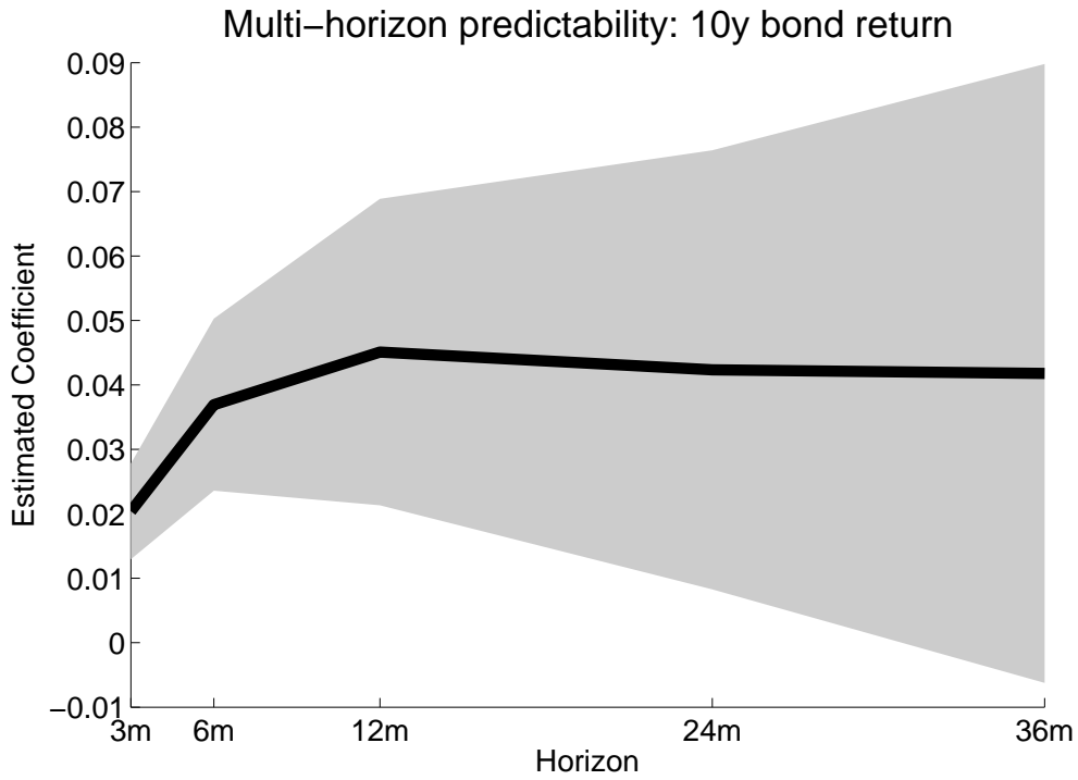
Figure 3. Multi-horizon predictability
