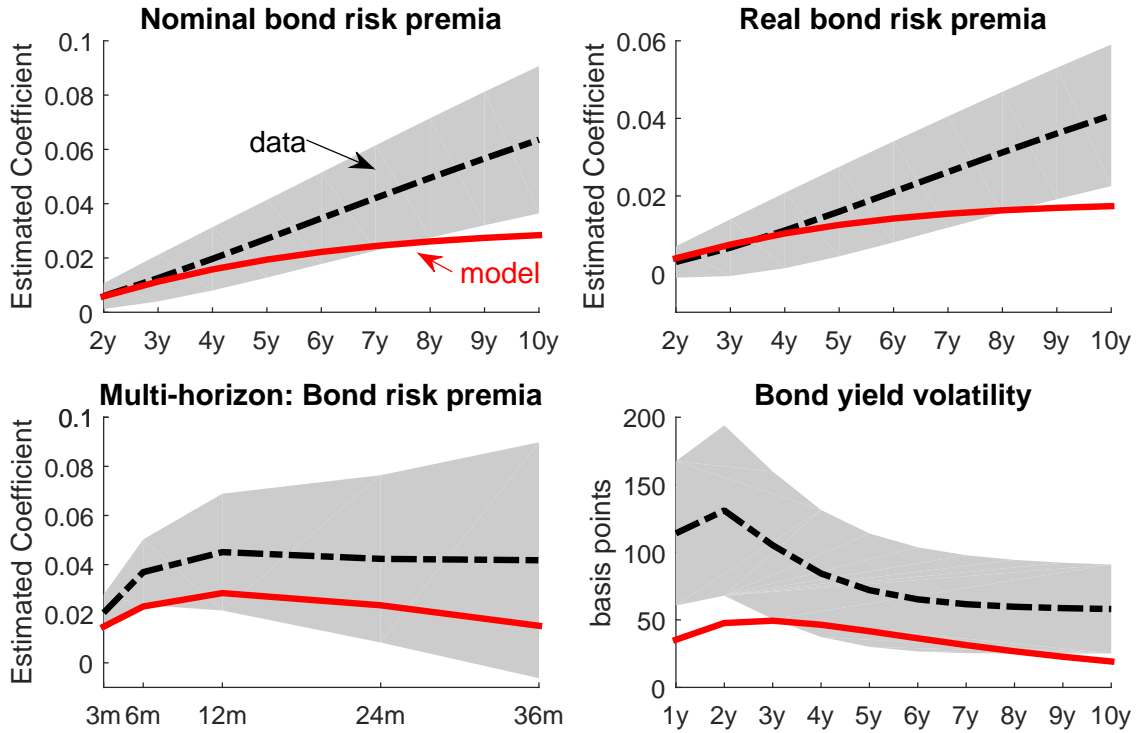
Figure 6. Calibration results
