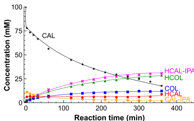
Figure 8. The outlet concentrations of the components obtained in the CAL hydrogenation as a function of residence time in a batch reactor. Reaction conditions: 0.1 g 12 wt % Pt/SiO 2 , H 2 pressure 10 bar, 90 °C, 0.1 M CAL in IPA.
