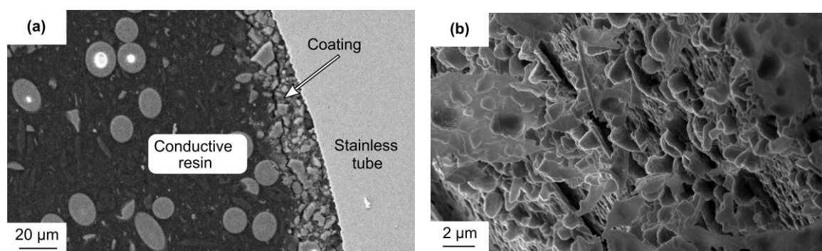
Figure 1. SEM (a) cross-sectional and (b) frontal images of the catalytic coating in a tube reactor.
