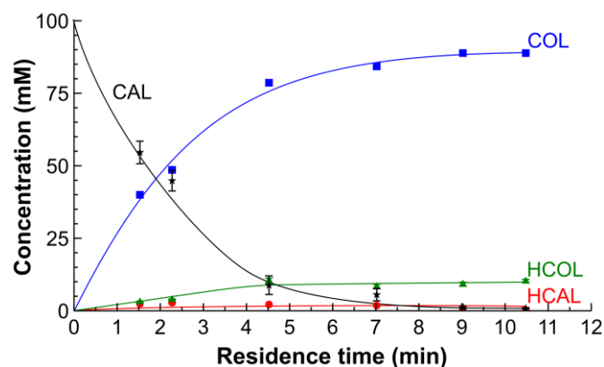
Figure 7. The outlet concentrations of the components obtained in the CAL hydrogenation as a function of residence time in the 5 m reactor coated with 190 mg 12 wt % Pt/SiO 2 catalyst. Reaction conditions: H 2 flow rate: 4–12 mL min −1 (standard temperature and pressure, STP), liquid flow rate: 0.2–3 mL min −1 , inlet CAL concentration: 0.1 M in IPA, pressure: 10 bar, temperature: 90 °C.
