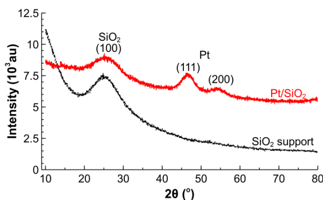
Figure 4. Powder X-ray diffraction patterns (using Co K α radiation) for the 12 wt % Pt/SiO 2 catalysts and the SiO 2 support.
