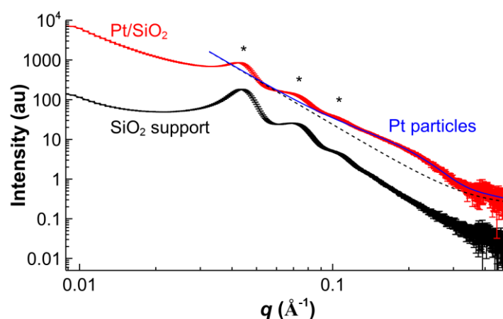
Figure 5. Small angle X-ray scattering obtained from the 12 wt % Pt/SiO 2 catalysts and the SiO 2 support. The overall fit for the Pt/SiO 2 is shown by the blue line and the fit without scattering from the Pt particles is given by the dashed line. The main features of SiO 2 is marked by *.
