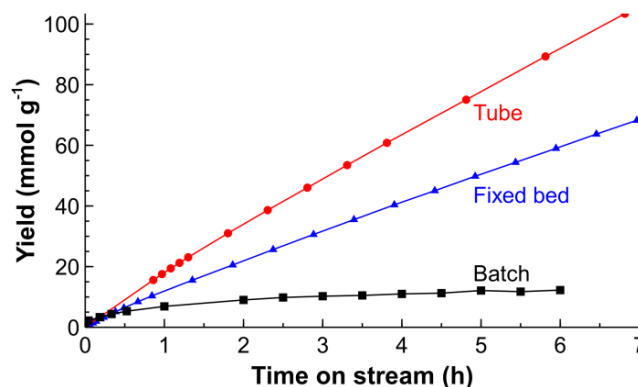
Figure 13. The comparison of cumulative COL yield over the Pt/SiO 2 catalysts in batch, fixed bed and tube reactors at the same condition (0.1 g 12 wt % Pt/SiO 2 , CAL concentration: 0.1 M in IPA, pressure: 10 bar and temperature: 90 °C).
