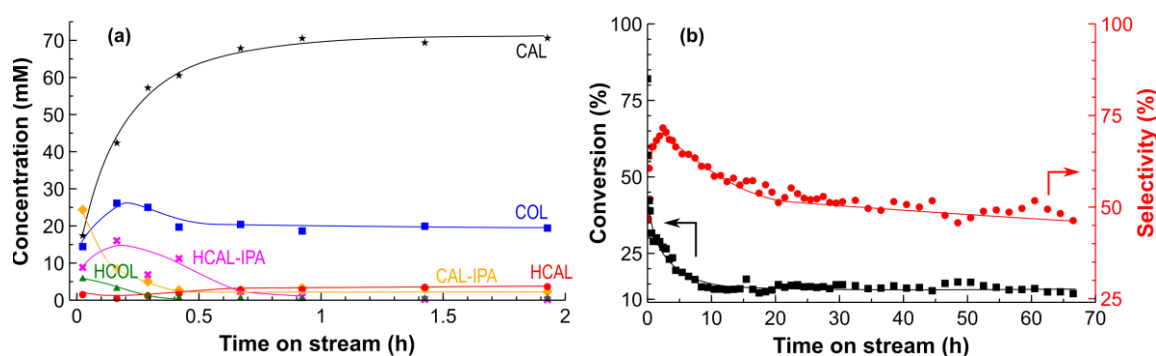
Figure 12. The stability test of a continuous fixed bed reactor packed with 190 mg 12 wt % Pt/SiO 2 . Reaction conditions: H 2 flow rate: 3 mL min −1 , liquid flow rate: 0.2 mL min −1 , CAL concentration: 0.8 M in IPA, pressure: 15 bar and temperature: 90 °C. (a) The outlet concentrations of the components obtained in the CAL hydrogenation as a function of time in stream. (b) The conversion of CAL and the selectivity to COL vs. Time on stream.
