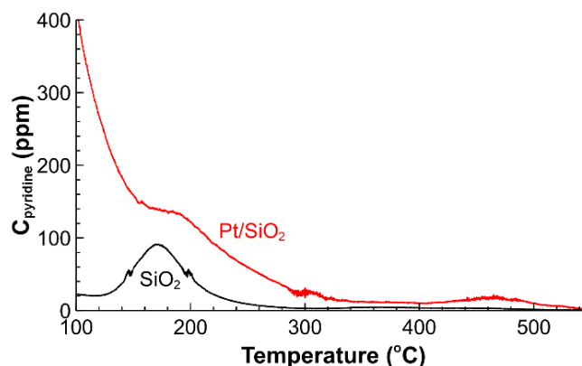
Figure 6. Temperature-programmed desorption profile of pyridine from the Pt/SiO 2 catalyst and SiO 2 support.
