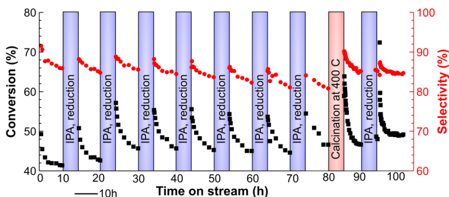
Figure 11. The stability test of the 2 m tube reactor coated with a 12 wt % Pt/SiO 2 catalyst. Reaction conditions: H 2 flow rate: 3 mL min −1 , liquid flow rate: 0.2 mL min −1 , CAL concentration: 0.8 M in IPA, pressure: 15 bar and temperature: 150 °C. Reduction was performed in the flow of isopropanol (1 mL min −1 ) and H 2 flow rate (3 mL min −1 , STP) for 10 min. Regeneration conditions: in air at 400 °C for 1 h. The duration of the reduction and calcination steps on the plot are exaggerated for the presentation purposes.
