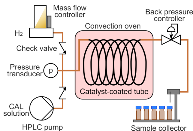
Figure 16. The scheme of the continuous flow hydrogenation system.
