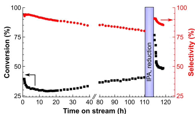
Figure 10. The stability test of the 5 m tube reactor coated with a 12 wt % Pt/SiO 2 catalyst. Reaction conditions: H 2 flow rate: 3 mL min −1 , liquid flow rate: 0.2 mL min −1 . CAL concentration: 0.8 M in IPA, pressure: 15 bar and temperature: 90 °C. Reduction was performed in the flow of isopropanol (1 mL min −1 ) and H 2 flow rate (3 mL min −1 , STP) for 10 min. The duration of the reduction step on the plot is exaggerated for the presentation purposes.
