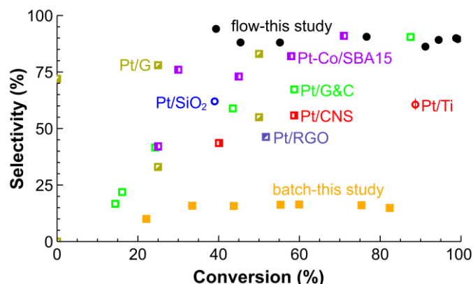
Figure 9. The selectivity to COL as a function of CAL conversion obtained in the current work over the 12 wt % Pt/SiO 2 catalyst in the tube (flow-this study, ●) and batch (batch-this study, ■) reactors compared with the literature data in obtained in continuous flow reactors (Pt/Ti, Φ [35]; Pt/SiO 2 ○ [31]) and batch reactors (Pt/G&C, □ [12]; Pt-Co/SBA-15, ▨ [19]; Pt/CNS, ▩ [23]; Pt/RGO, ▤ [53]; Pt/G, ▧ [54]). Circles represent continuous flow and squares represent batch reactors.
