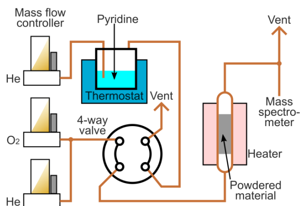
Figure 15. The scheme of the setup used for the pyridine chemisorption study.
