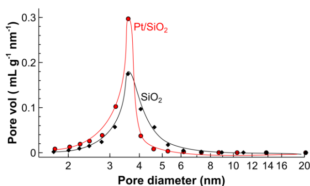
Figure 3. Barrett–Joyner–Halenda (BJH) desorption pore-size distribution for the SiO 2 support and Pt/SiO 2 catalyst studied.
