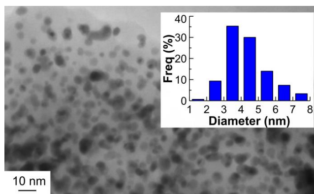
Figure 2. TEM image of the Pt nanoparticles supported on SiO 2 with their diameter distribution.
