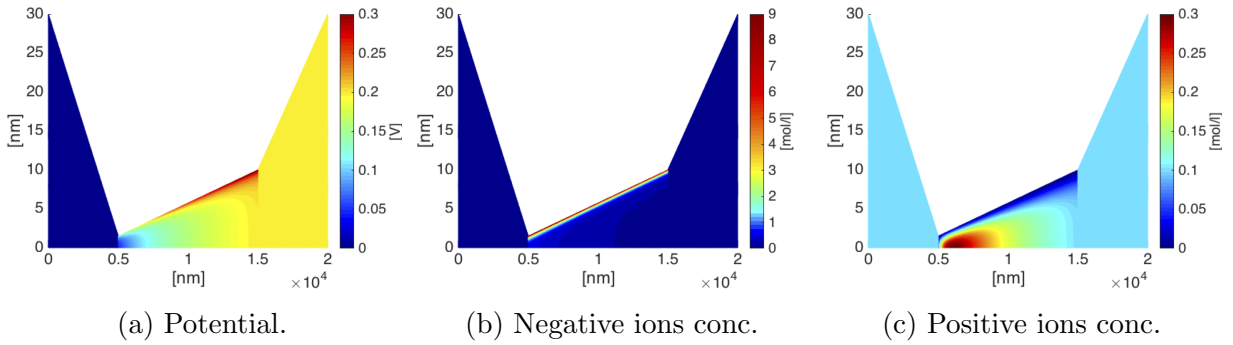
Figure 9: Heat maps of the potential and two ionic concentrations obtained using the 2D PNP solver for the conical pore.
