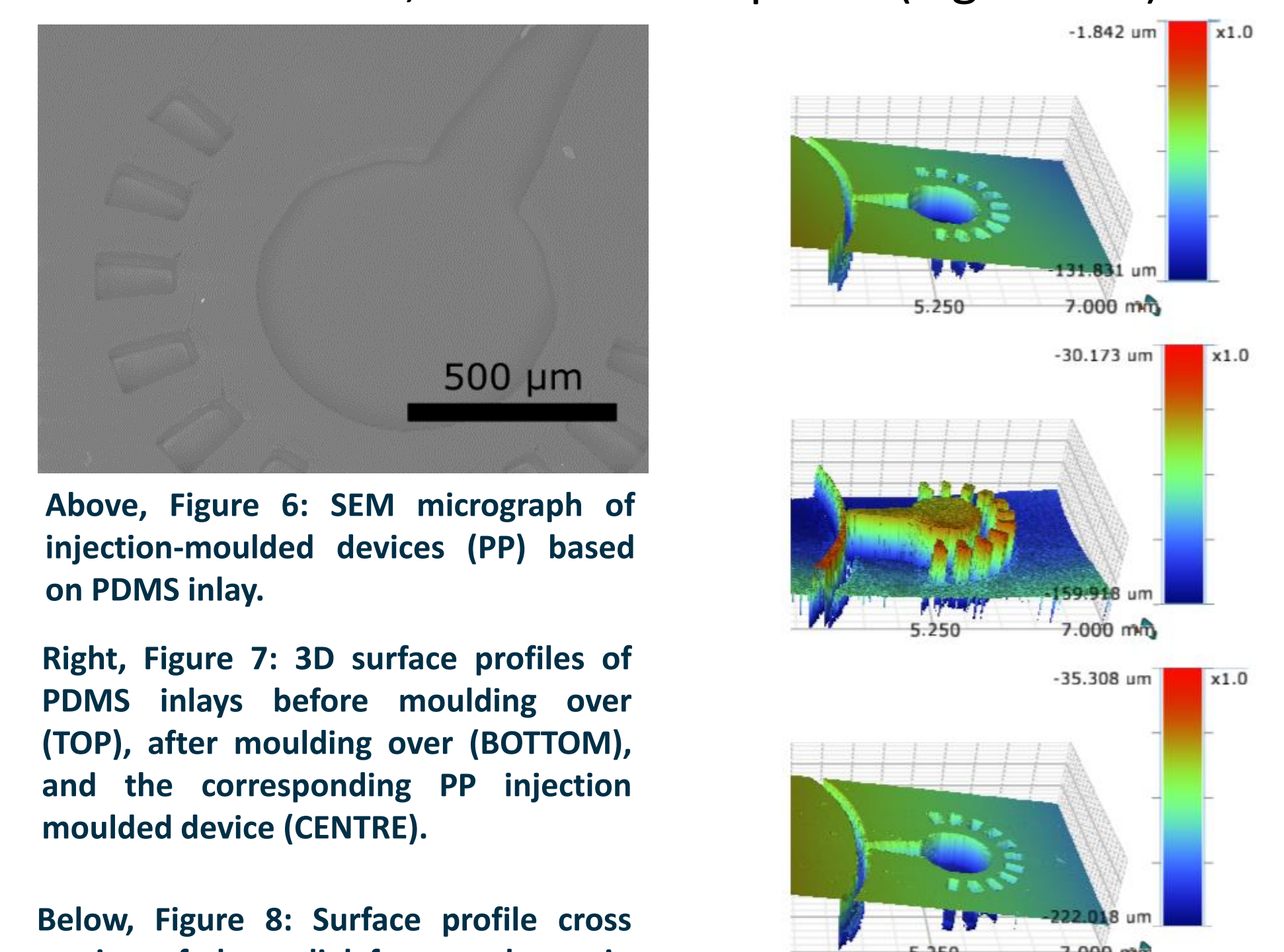
Figure 7: 3D surface profiles of PDMS inlays before moulding over (TOP), after moulding over (BOTTOM), and the corresponding PP injection moulded device (CENTRE).
