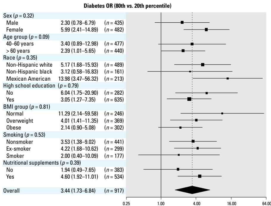
Figure 2. Adjusted ORs (95% CIs) for diabetes comparing the 80th percentile (150 \mu\text{g/L} ) with the 20th percentile (122 \mu\text{g/L} ) of the serum selenium distribution. Serum selenium was modeled as restricted quadratic splines with nodes at the 5th, 50th, and 95th percentiles. Multivariable logistic regression models were adjusted for sex, age, race, education, BMI, smoking, cotinine, postmenopausal status, and use of vitamin and mineral supplements (model 3). The size of the square indicates the number of participants in each stratum. p -Values correspond to tests for interaction between selenium splines and selected participant characteristics.
