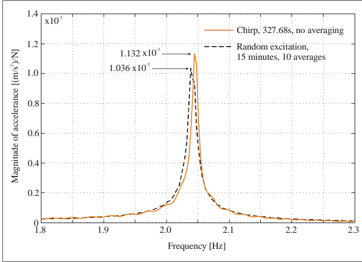
Figure 14: Magnitude of acceleration in the first vertical mode of vibration due to two different types of excitation.
