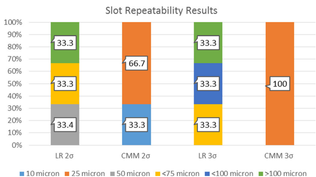
Fig. 12 Repeatability of slot measurement results for LR and CMM
