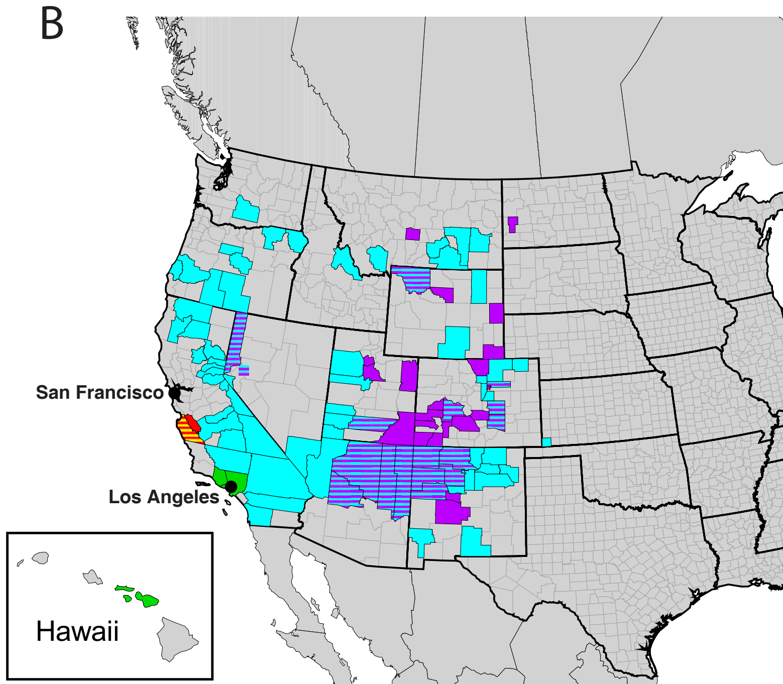
Supplementary Figure 4. Expansion of plague in the U.S.A. A) MSTree segment of radiation 1.ORI1. SNPs that define individual steps (s57, s429, etc.) are shown in grey. Node sizes correlate with the numbers of isolates assigned to those nodes (parentheses). B) Map of the U.S.A. showing the distribution of isolates by county, color-coded according to node in part A.
