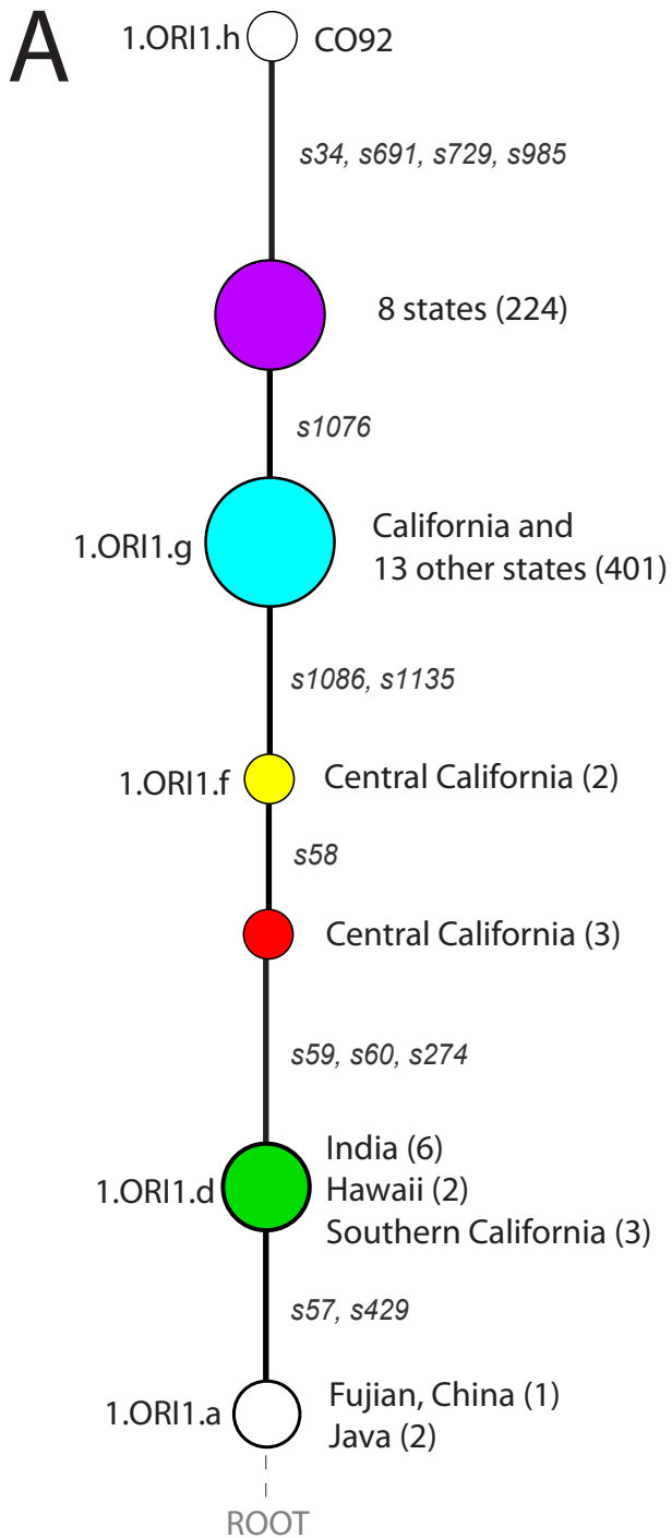
Supplementary Figure 4. Expansion of plague in the U.S.A. A) MSTree segment of radiation 1.ORI1. SNPs that define individual steps (s57, s429, etc.) are shown in grey. Node sizes correlate with the numbers of isolates assigned to those nodes (parentheses). B) Map of the U.S.A. showing the distribution of isolates by county, color-coded according to node in part A.
