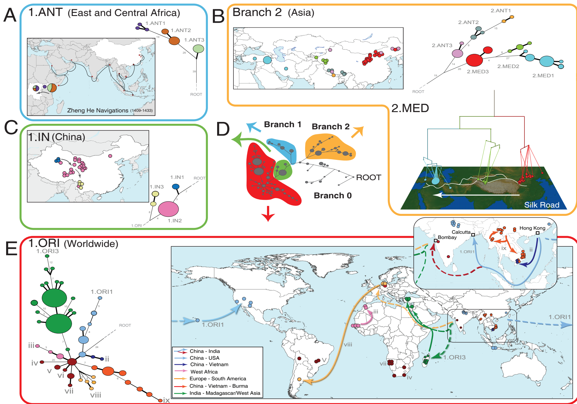
Supplementary Figure 3. Postulated routes of spread. D) A condensed MSTree ( Fig. 2 ) with colored sections that are repeated in parts A-C and E, within which corresponding colors link locations within maps (circles, pie charts) to nodes within the MSTree segment. A) Sources of 1.ANT isolates in Central Africa and routes of navigation (black lines) by Zheng He from China to Africa in 1409-1433. B) upper left: sources of isolates from branch 2 superimposed on a map of Asia. lower right: sources of 2.MED isolates superimposed on a topographical map of the Silk Road (white lines; 200 BC – 1,400). C) Direction of spread of 1.IN nodes within China from northwest to south. E) Postulated routes of migration of 1.ORI since 1894. ii – ix: Radiations with few isolates. Radiations 1.ORI1 and 1.ORI3 are expanded in Supplementary Figs. 4-5 .
